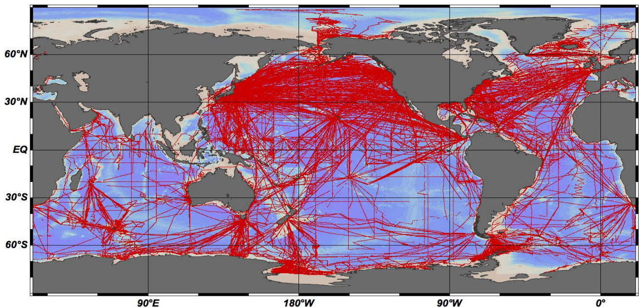
Fig. 1. Location of LDEO V2016 master database of sea surface pCO 2 observations.
