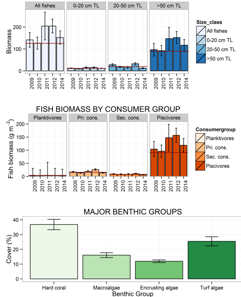
Figure 35 Lisianski Island fish and benthic plots showing the biomass (g m -2 ± SE) of fish observed in total and per size class (top) and per consumer group (middle) and the percentage cover (± SE). The benthic estimates are pooled across all years. The Northwestern Hawaiian Islands region mean estimates are plotted for reference (red line).
