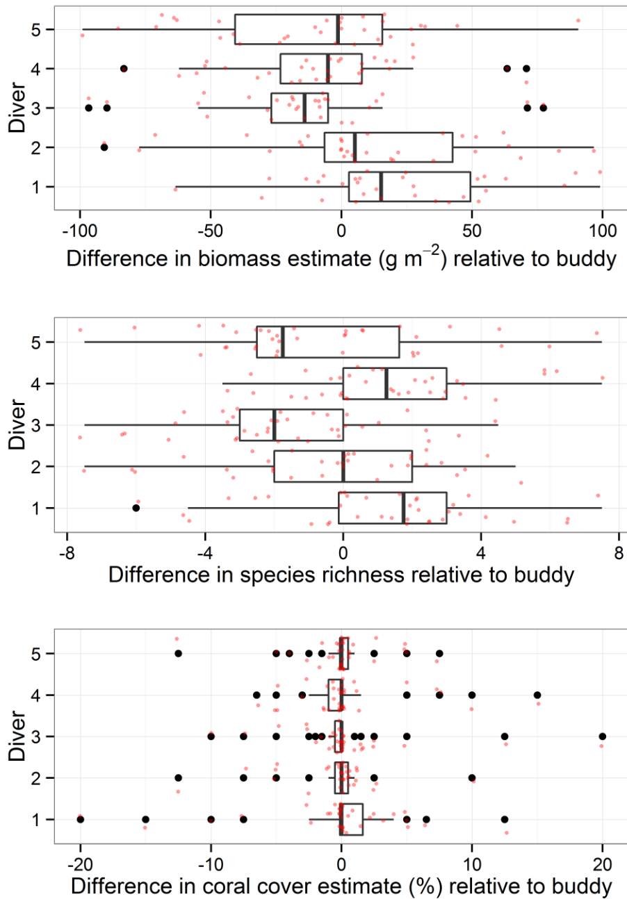
Figure A5.4 Northwestern Hawaiian Islands comparison of observer diver vs dive partner estimates for total fish biomass, species richness and hard coral cover during 2014 surveys. See Figure A5.2 legend for details. Note that the 2014 survey cruise in the NWHI was led by the PMNM. Although methods and design are identical between CRED and PMNM cruises, PMNM cruises involve divers with a wider range of experience levels than is typical for CRED cruises.
