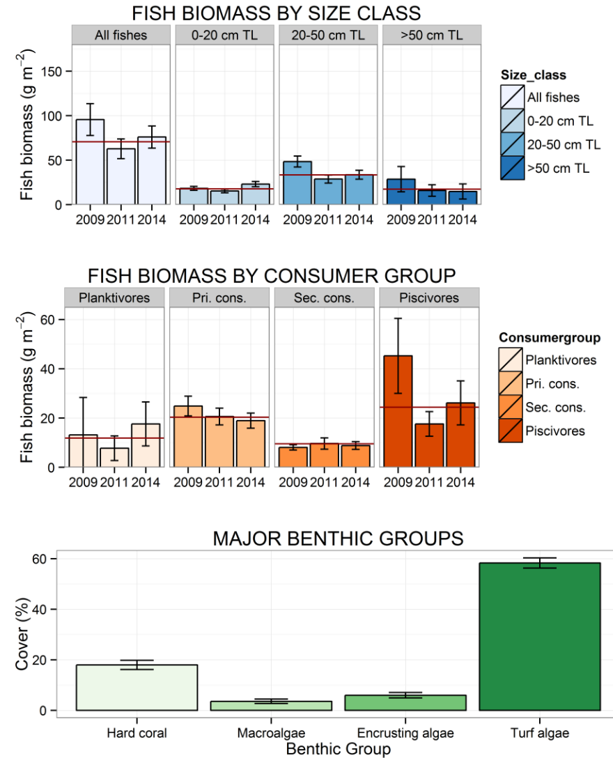
Figure 10 Asuncion Island fish and benthic plots showing the biomass ( \text{g m}^{-2} \pm \text{SE} ) of fish observed in total and per size class (top) and per consumer group (middle) and the percentage cover ( \pm \text{SE} ) of the benthos. The benthic estimates are pooled across all years. The northern Mariana region mean estimates are plotted for reference (red line).
