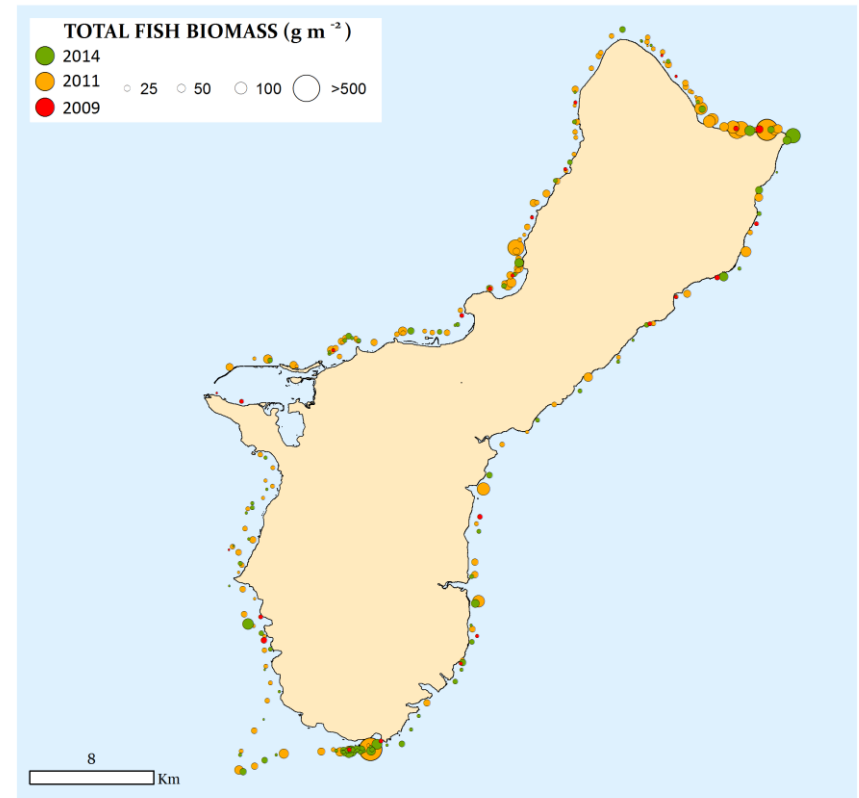
Figure 20 Total fish biomass recorded at each site per year.
