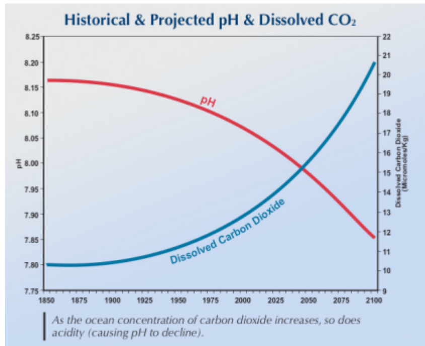
Figure 11. Current and Future Ocean Acidification Estimates (Feeley et al. 2006)
