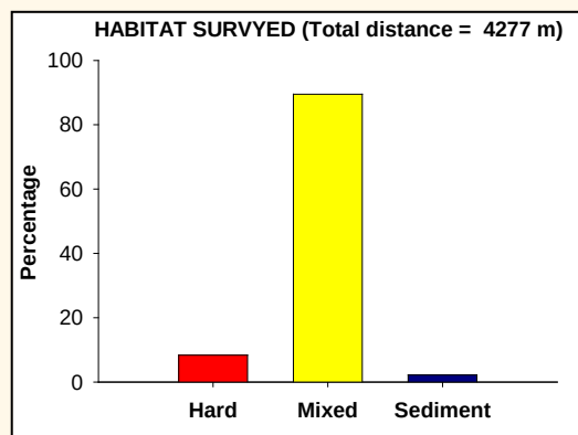
Figure 5. Percent habitat (hard, mixed, sediment) observed along qualitative segments.
