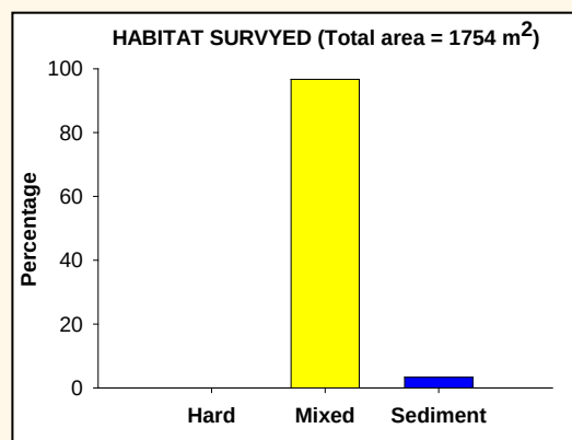
Figure 4. Percent habitat (hard, mixed, sediment) observed along quantitative segments.
