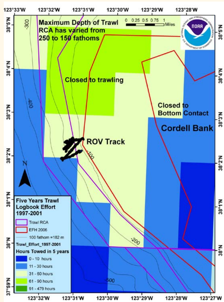
Figure 6. Total hours of bottom trawl tows, 1997-2001, per 1 minute 2 microblock
