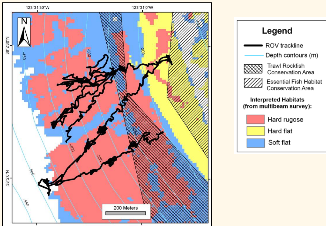
Figure 1(b). ROV trackline overlaid on interpreted habitats at dive site
