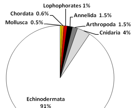
TOTAL DENSITY OF SMALL INVERTEBRATES 1036 small invertebrates/1,000 m 2
