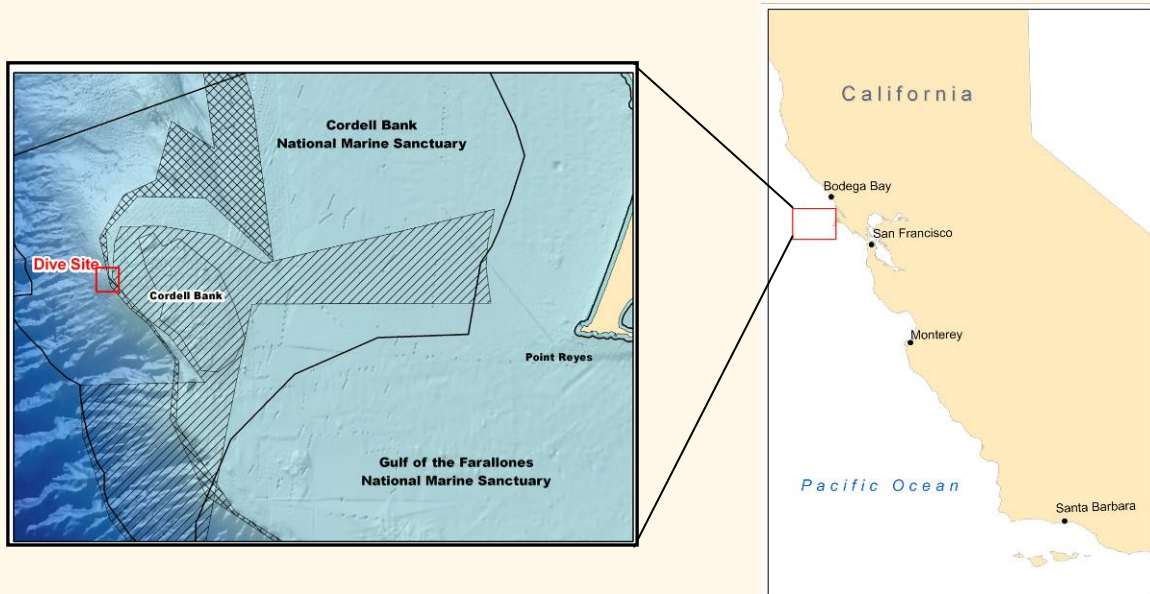
Figure 1(a). Location of ROV dive site on the continental slope west of Cordell Bank, northern California
