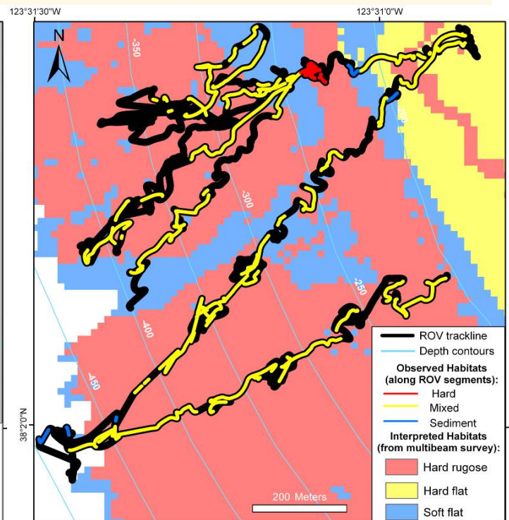
Figure 3. Habitat types observed along ROV segments
