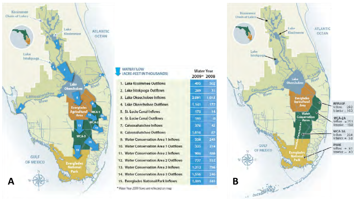
Figure 30: A) Year 2009 water flows (1000 acre-feet) along the Kissimmee-Okeechobee-Everglades watershed. B) Water year 2009 mean phosphorus concentrations (ppb) (inflows are flow-weighted mean concentrations, interiors are geometric mean concentrations) (SFWMD, 2010).
