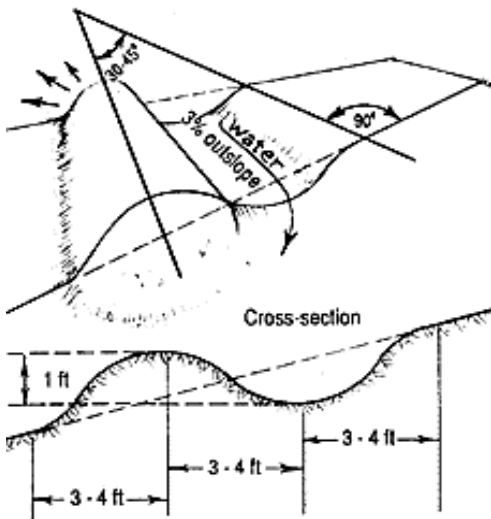
Waterbar Cross Section (Source: MN Extension Service)
