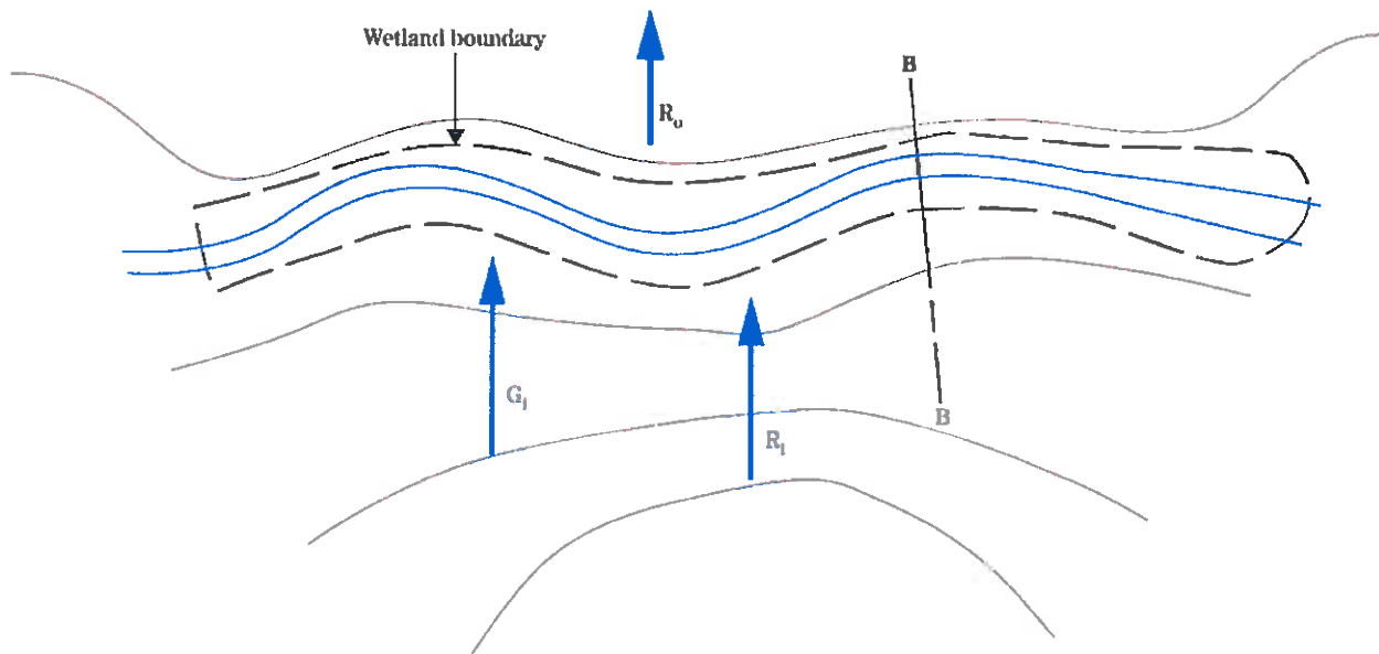
Figure 3 – Stratigraphic Slope HGM Wetland Class Plan View
