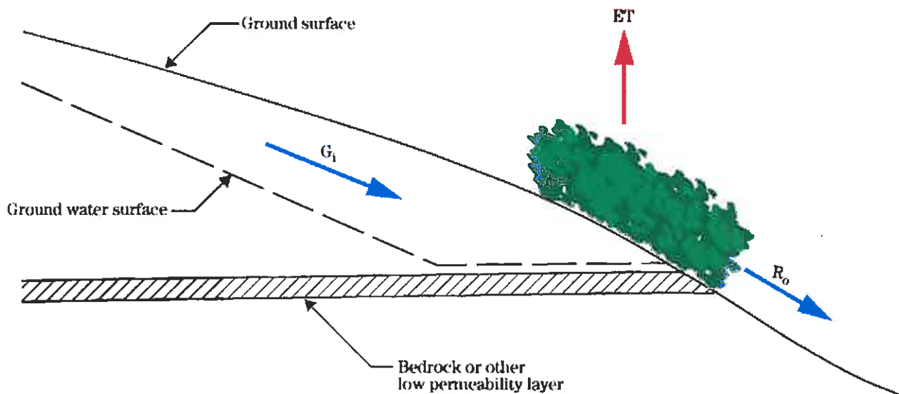
Figure 4 – Stratigraphic Slope HGM Wetland Class Section B-B
