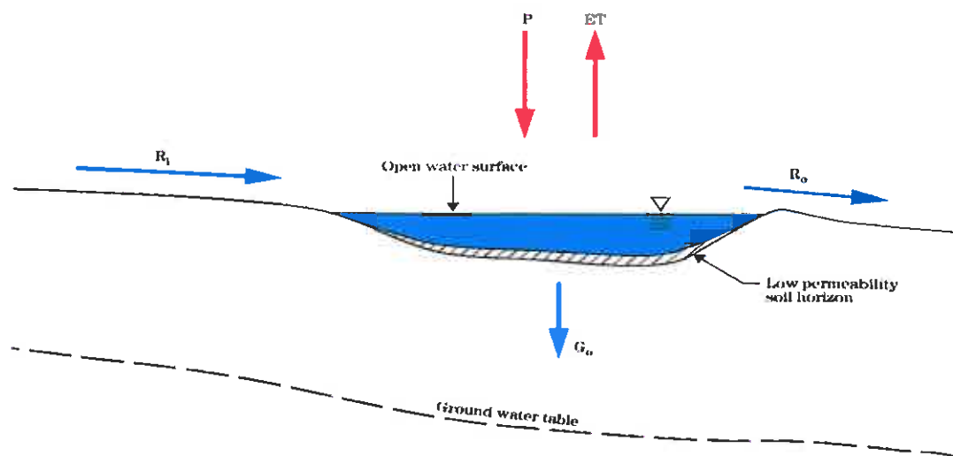
Figure 1 – Hydrodynamics of Recharge Depressional Wetlands
