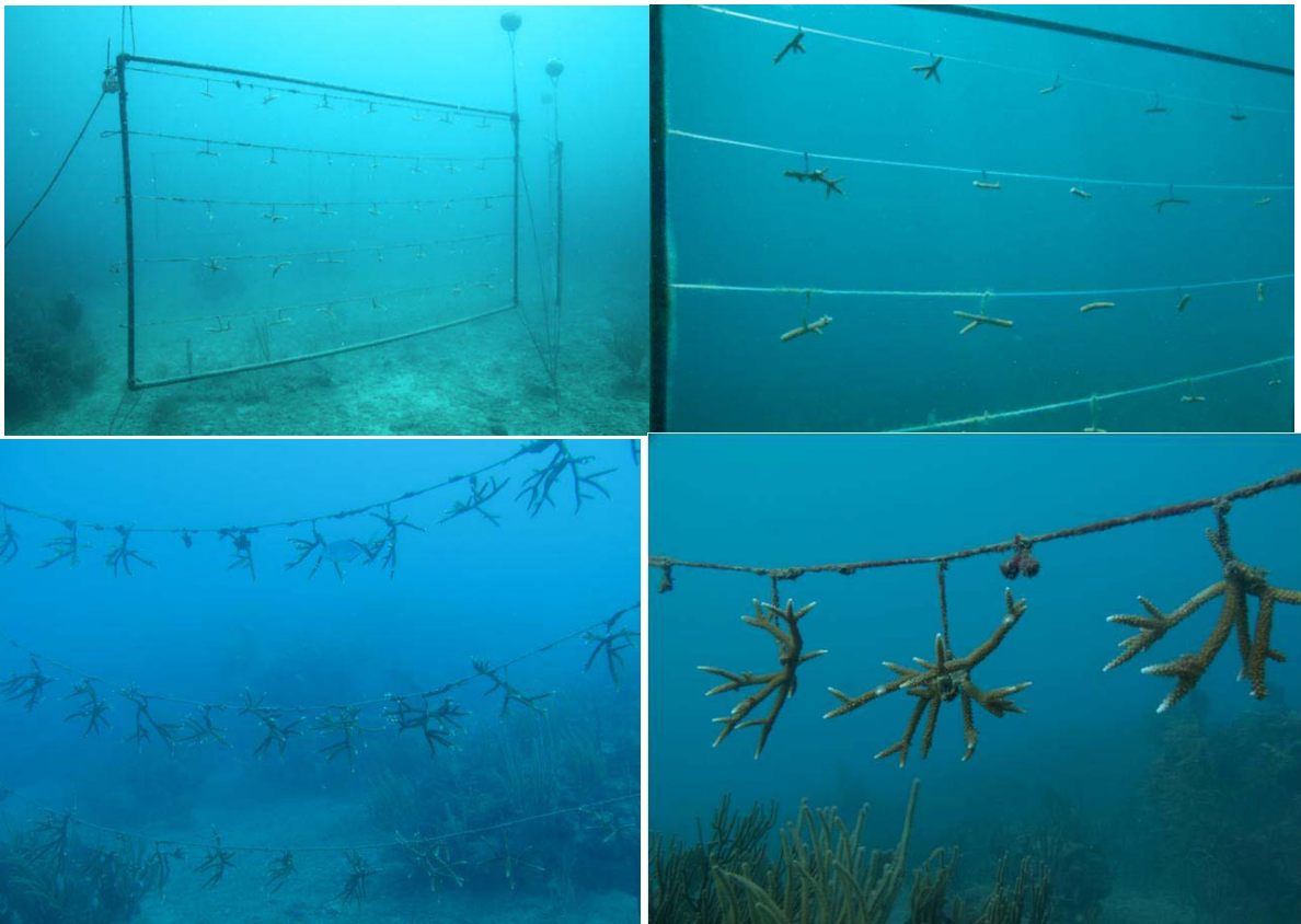
Figure 3: Photos showing a typical 5' x 10' line nursery set up with 5 cm coral fragments (top) and 12 months of coral growth on a line nursery with 25 cm colonies (bottom).
