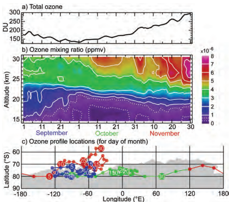
FIG. 6.10. OMPS ozone observations from a location near the center of the polar vortex: (a) total column ozone (in DU) and (b) daily ozone profiles (in ppmv). Values have been smoothed in time using a 1-2-1 filter. (c) The circles show vortex daily location with every fifth day numbered. The blue, green, and red circles indicate Sep, Oct, and Nov, respectively.
