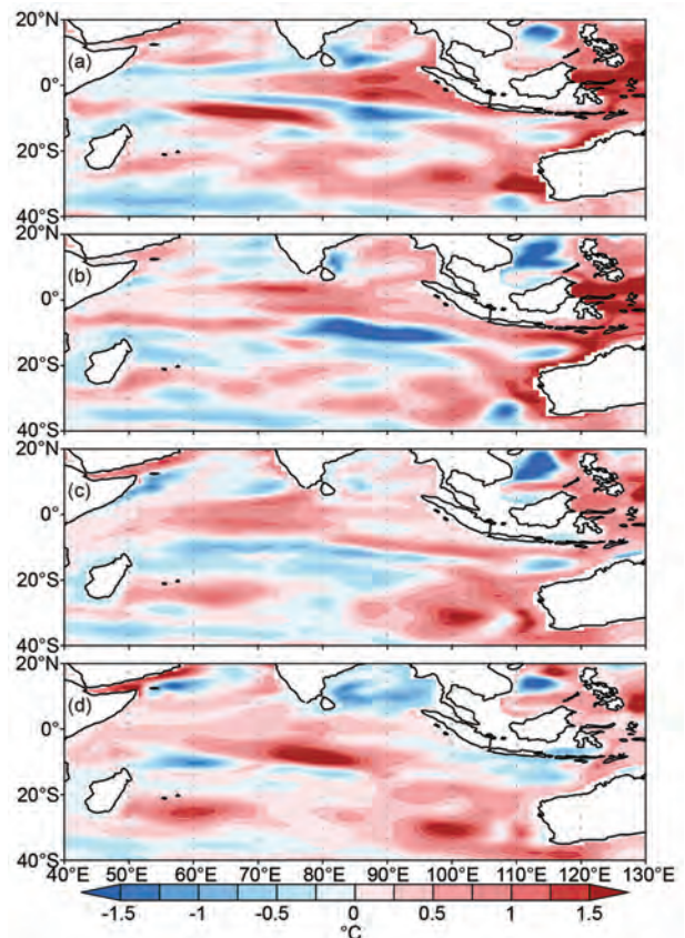
FIG. 4.39. Upper 300 m mean ocean temperature anomalies ( ^{\circ}\text{C} ) based on the NCEP ocean reanalysis during (a) DJF2011/12, (b) MAM 2012, (c) JJA 2012, and (d) SON 2012. (Source: www.cpc.ncep.noaa.gov/products/GODAS/ .)
