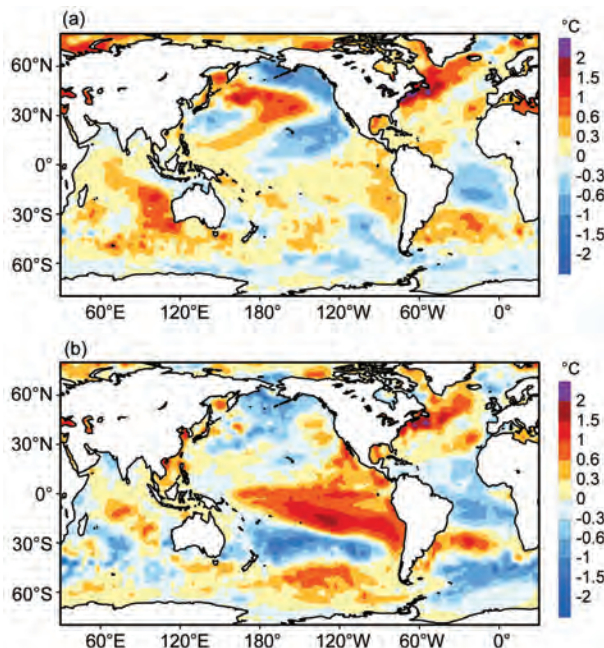
FIG. 3.1. (a) Yearly mean OISST anomaly (°C, relative to 1981–2010 average) in 2012; (b) 2012 minus 2011 OISST anomaly.
