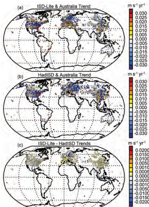
FIG. 2.26. Global distributions of the land wind speed trends ( \text{m s}^{-1} \text{ yr}^{-1} ) for 1981–2012 calculated using (a) the augmented NOAA ISD-LITE database and (b) augmented HadISD dataset. (c) Trend differences between the two, calculated as (a)-(b).
