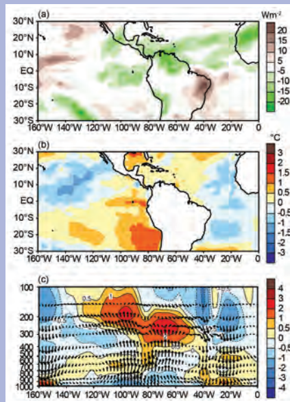
FIG. SB.7.3. (a) Anomalous outgoing longwave radiation (OLR, \text{W m}^{-2} ), (b) sea surface temperatures (SSTs, ^{\circ}\text{C} ), and (c) zonal divergent circulation, for Feb–Apr 2012. (Source: NCEP/NCAR.)
