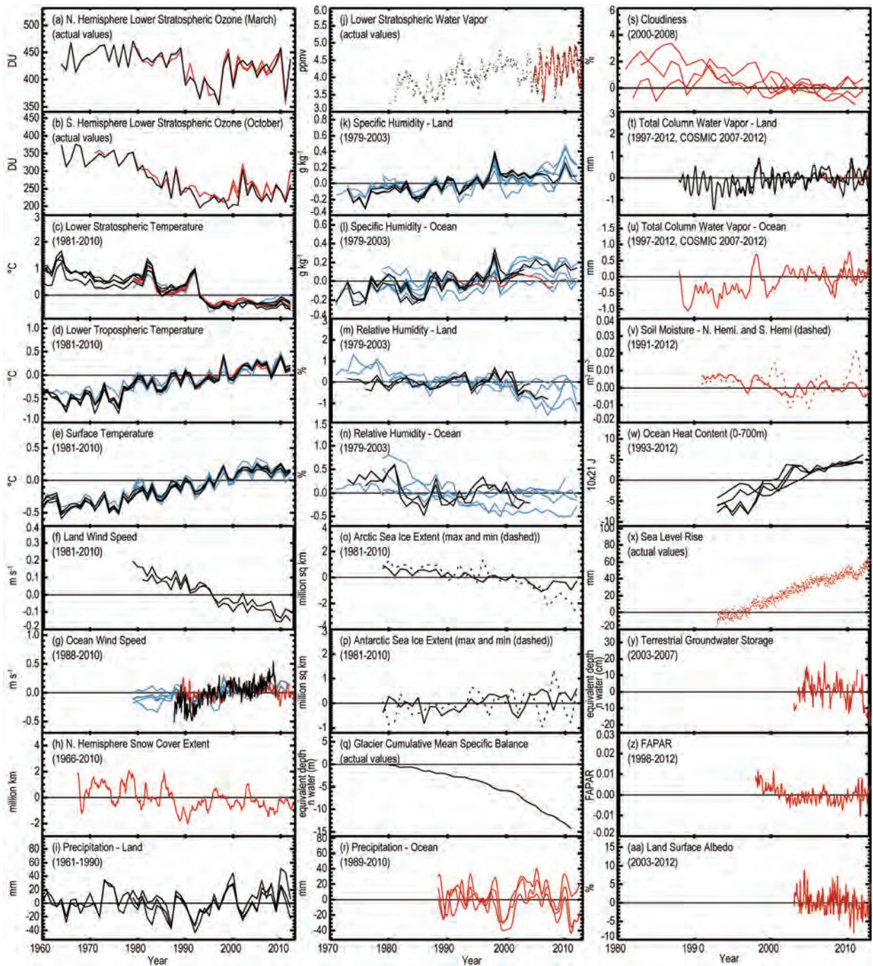
PLATE I.1 Global (or representative) average time series for essential climate variables. Anomalies are shown relative to the base period in parentheses although original base periods may differ. Data products are colored black for in situ (IS), red for satellite (S), and blue for reanalyses (R). (a) Northern Hemisphere lower stratospheric ozone in March (IIS, 2S); (b) Southern Hemisphere lower stratospheric ozone in October (IIS, 2S); (c) Lower stratospheric temperature (4IS, 3S, 3R); (d) Lower tropospheric temperature (4IS, 2S, 4R); (e) Surface temperature (4IS, 5R); (f) Land surface wind speed (2IS); (g) Ocean surface wind speed (IIS, IS, 5R); (h) Northern Hemisphere continental snow cover extent (IS); (i) Precipitation over land (3IS); (j) Lower stratospheric water vapor over Boulder, CO (IIS, IS); (k) Surface specific humidity over land (4IS, 5R); (l) Surface specific humidity over ocean (3IS, 5R); (m) Surface relative humidity over land (3IS, 4R); (n) Surface relative humidity over ocean (2IS, 4R); (o) Arctic sea ice extent (IIS); (p) Antarctic sea ice extent (IIS); (q) Glacier cumulative mean specific balance (IIS); (r) Precipitation over ocean (3S); (s) Cloudiness (IIS, 5S); (t) Total column water vapor over land (2IS, IS); (u) Total column water vapor over ocean (2S[kI]); (v) Soil moisture (IS); (w) Ocean heat content (0–700m) (4IS); (x) Sea level rise (IS); (y) Terrestrial groundwater storage (IS); (z) FAPAR (IS); (aa) Land surface albedo in the visible spectrum (IS).
