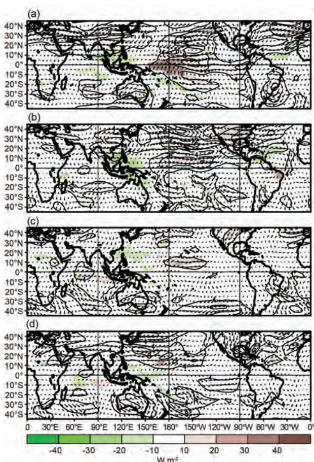
FIG. 4.6. Anomalous 200-hPa wind vector and speed (contours, \text{m s}^{-1} ) and anomalous OLR (shaded, \text{W m}^{-2} ) during (a) DJF 2011/12, (b) MAM 2012, (c) JJA 2012, and (d) SON 2012. Anomalies are departures from the 1981–2010 monthly means.
