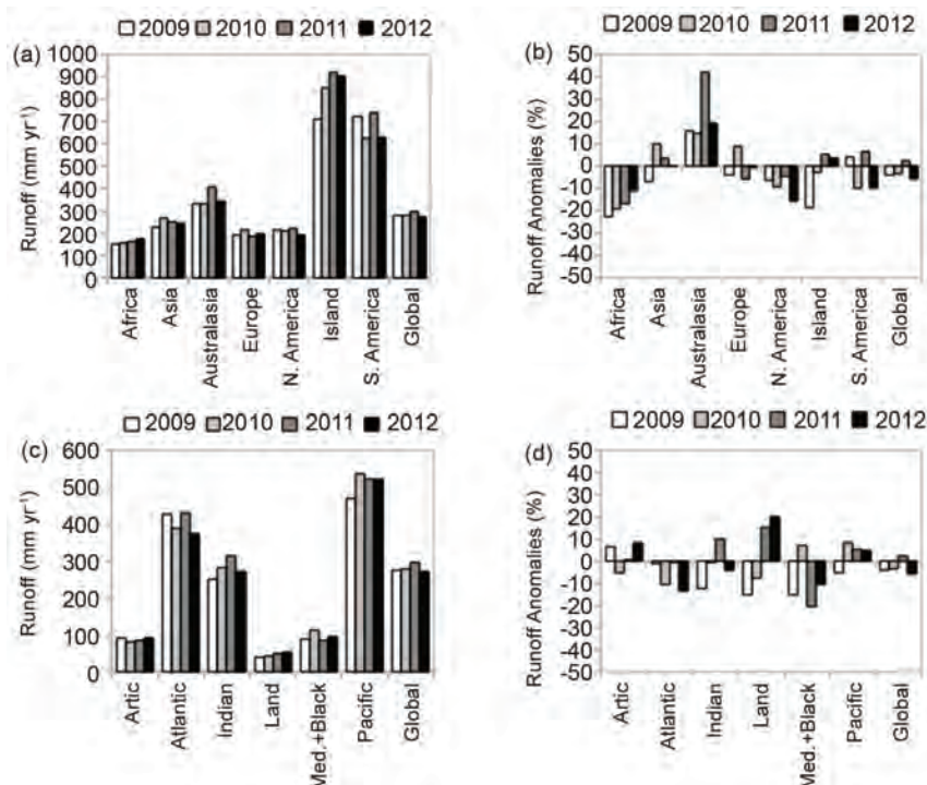
FIG. 2.16. Water Balance Model runoff estimates: (a), (b) over continents and (c), (d) by receiving oceans. (a), (c) Annual runoff and (b), (d) annual anomalies (relative to 1948–2010) for 2009, 2010, 2011, and 2012.
