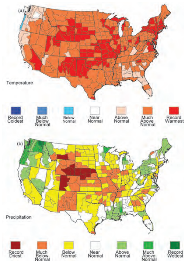
FIG 7.6. Climate division ranks of annual 2012 (a) temperature and (b) precipitation. Record coldest/warmest or driest/wettest is defined as the smallest/largest annual value for that climate division in the 1895–2012 period of record. Above-normal temperature/precipitation is defined as occurring in the warmest/wettest third of recorded years. Whereas, much-below-normal temperature/precipitation falls in the bottom 10% of coolest/driest years since 1895, and below normal is defined as the coolest/driest third of the distribution. (Source: NOAA/NCDC.)
