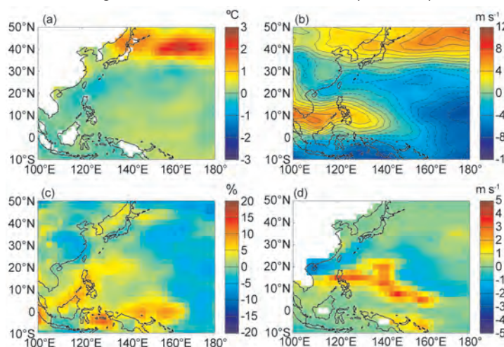
FIG. 4.21. (a) SST anomalies for Jul–Oct (JASO) 2012. (b) Zonal winds in JASO 2012 (positive contours are shown in solid lines, negative contours in dash dotted lines, and the zero contour in a dotted line). (c) Relative humidity 600-hPa anomalies in JASO 2012. (d) Genesis potential index anomalies in JASO 2012. [Source: atmospheric variables: NCEP/NCAR Reanalysis data (Kalnay et al. 1996); SSTs (Smith and Reynolds 2005).]
