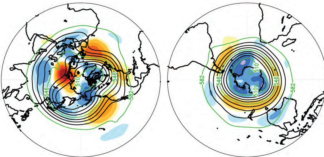
FIG. AI.2. Dec 2011–Feb 2012 (top) Northern Hemisphere and (bottom) Southern Hemisphere 500 hPa geopotential heights (9-dam contour interval) and anomalies (shading) determined from the 1981–2010 base period means. Data is from the CDAS/Reanalysis Project (Kalnay et al. 1996).
