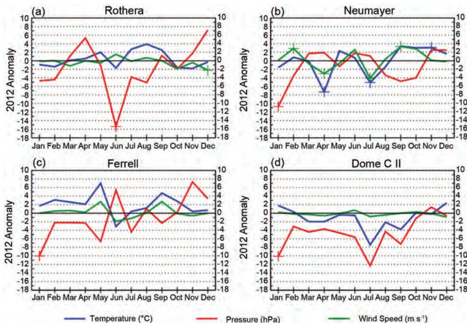
FIG. 6.5. (a)–(d) 2012 Antarctic climate anomalies at four representative stations [two staffed: (a) and (b), and two automatic: (c) and (d)]. Monthly mean anomalies for temperature ( ^{\circ}\text{C} ), MSLP (hPa), and wind speed ( \text{m s}^{-1} ) are shown, + denoting record anomalies for a given month at each station in 2012. Climatological data start in 1976 for Rothera, 1981 for Neumayer and Ferrell, and 1980 for Dome C II. The base period for calculating anomalies is 1981–2010 for all stations.
