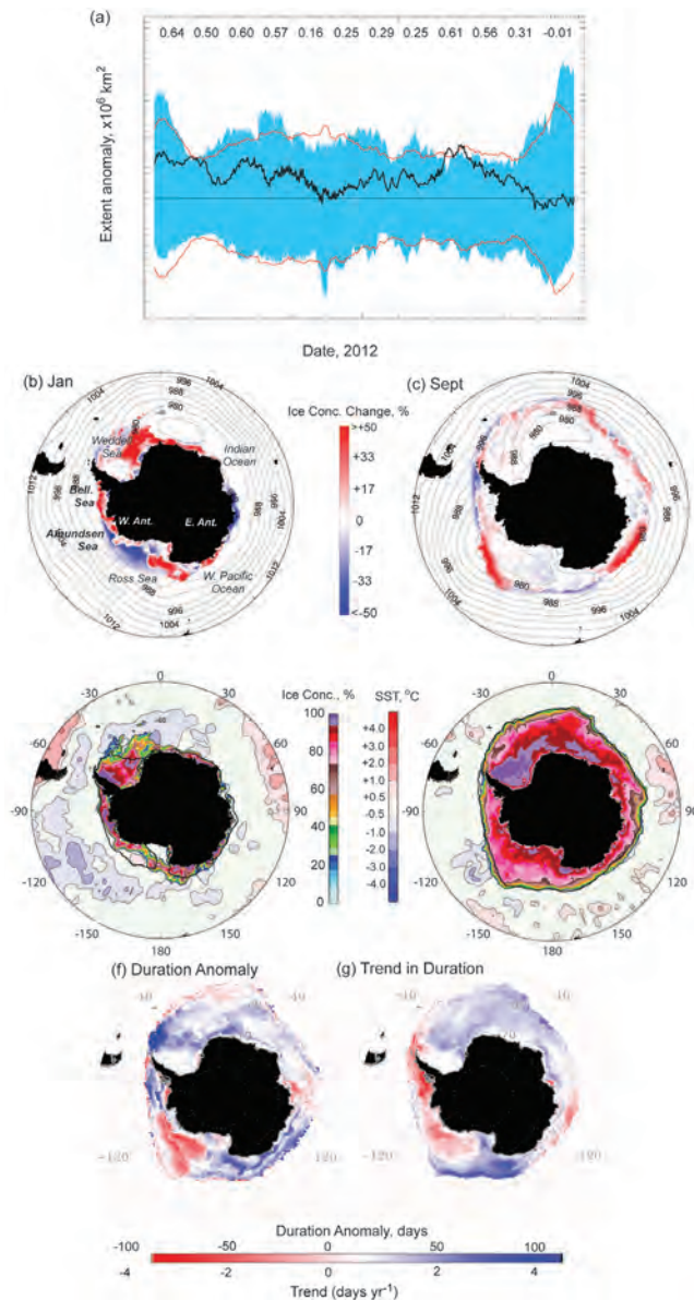
FIG. 6.8. a) Plot of daily anomaly (black line) from the 1981–2010 mean of daily SH sea ice extent for 2012, based on satellite passive microwave ice concentration data from the GSFC Bootstrap Version 2 dataset (Comiso 2008). Blue banding represents the range of daily values for 1981–2010, while the red line represents \pm 2 std devs. Numbers at the top are monthly-mean extent anomalies ( \times 10^6 \text{ km}^2 ). (b) and (c) Sea ice concentration anomaly maps for Jan and Sep 2012 derived versus the monthly means for 1981–2010, with monthly-mean contours of ACCESS MSLP. Bell is Bellingshausen Sea. (d) and (e) Maps of monthly-mean sea ice concentration for Jan and Sep 2012, respectively, with mean ice edge/extent contours for 1981–2010 (black lines) and SST anomaly contours superimposed. The SST anomalies were calculated against the 1981–2010 mean and are based on data from the Optimal Interpolation SST version 2 dataset (Reynolds et al. 2002; Smith et al, 2008). (f) Sea ice duration anomaly for 2012/13, and (g) duration trend (see Stammerjohn et al. 2008). Both the climatology (for computing the anomaly) and trend are based on 1981/82 to 2010/11 data (Comiso 2008), while the 2012/13 duration-year data are from the NASA Team Near-Real-Time Sea Ice (NRTSI) dataset (Maslanik and Stroeve 1999).
