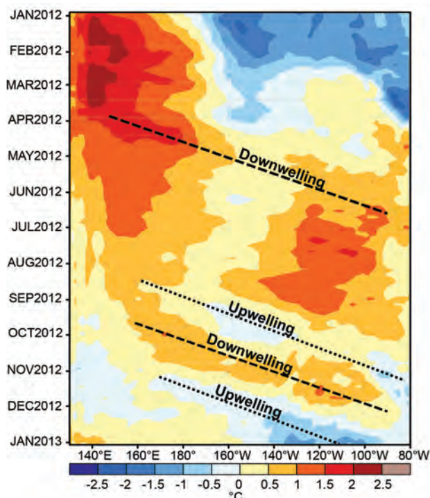
FIG. 4.8. Time-longitude section for 2012 of the anomalous upper Pacific Ocean (0–300 m) heat content averaged between 5°N–5°S. Blue (yellow/red) shading indicates below (above) average heat content. The downwelling (dashed lines) and upwelling (dotted lines) phases of equatorial oceanic Kelvin waves are indicated. Anomalies are departures from the 1981–2010 pentad means.
