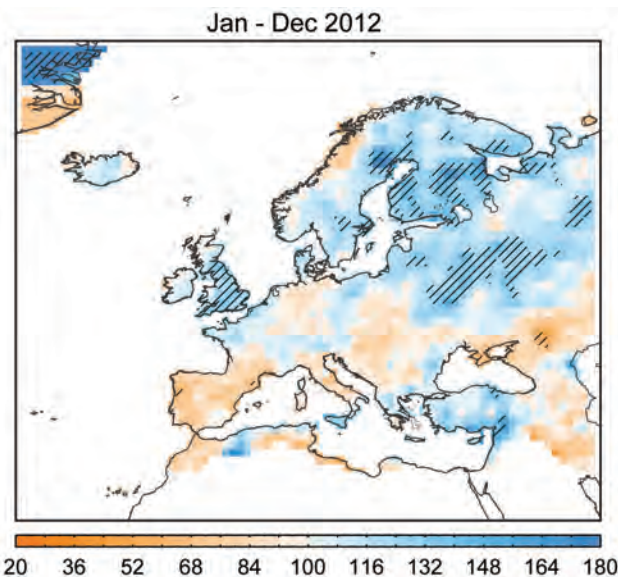
FIG. 7.31. European precipitation totals (% of normal, 1961–90 base period) for 2012. Hatched areas indicate regions where precipitation is higher (lower) than the 95th percentile (5th percentile) of the 1961–90 distribution. Only grid points with annual normals above 15 mm month -1 are represented. [Source: Global Precipitation Climatology Centre (Schneider et al. 2011b)].
