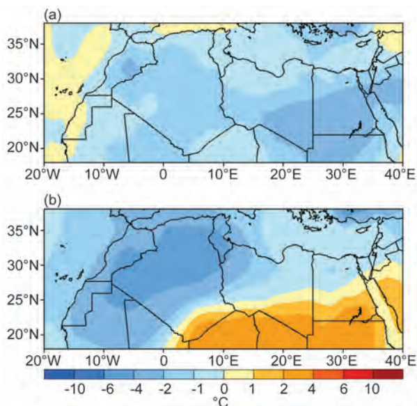
FIG. 7.17. Temperature anomaly ( ^{\circ}\text{C} ) in northern Africa in (a) Jan 2012 and (b) Feb 2012 departure from the 1981–2010 mean. (Source: NOAA/NCEP.)
