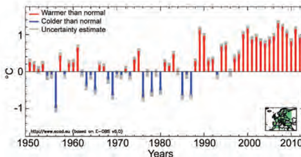
FIG. 7.30. Annual land surface air temperature anomaly (°C) for Europe, similar to Fig. 7.29, but based on the E-OBS dataset (van der Schrier et al. 2013) from 1950 to 2012. [Source: KNMI (Royal National Meteorological Institute) Netherlands.]
