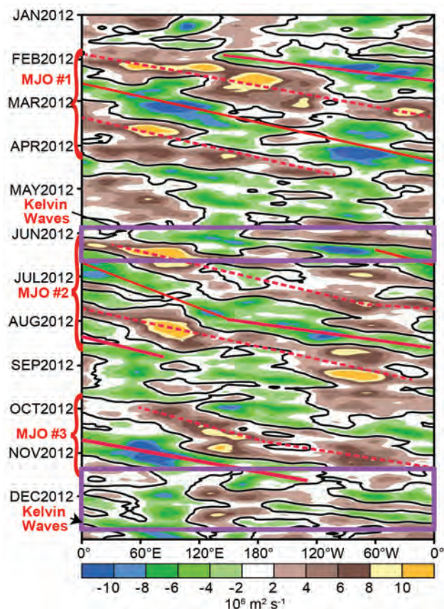
FIG. 4.7. Time-longitude section for 2012 of anomalous 200-hPa velocity potential ( \times 10^6 \text{ m}^2 \text{ s}^{-1} ) averaged between 5^\circ\text{N} – 5^\circ\text{S} . For each day, the period mean is removed prior to plotting. Green (brown) shading highlights likely areas of anomalous divergence and rising motion (convergence and sinking motion). Red lines and labels highlight the main MJO episodes. Purple boxes denote periods of atmospheric Kelvin wave activity discussed in text. Anomalies are departures from the 1981–2010 base daily means.
