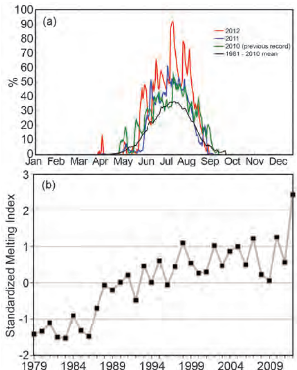
Fig. 5.13. (a) Surface melt extent, detected by the SSM/I passive microwave sensor, expressed as % of the total area of the Greenland Ice Sheet. (b) Standardized melt index (SMI) for the period 1979–2012 using the Tedesco (2009) algorithm.
