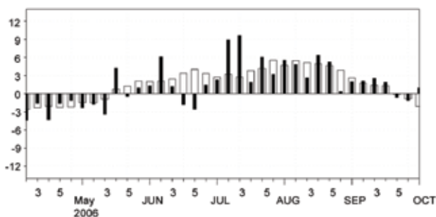
FIG. 6.30. Variation of the zonal wind index over the South China Sea ( \text{m s}^{-1} ).
