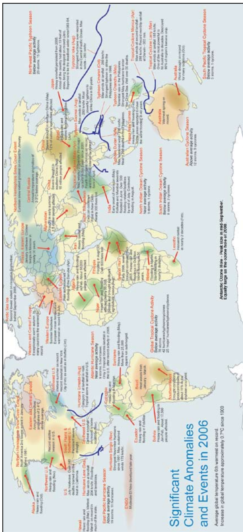
Fig. 1.1. Geographical distribution of notable climate anomalies and events occurring around the planet in 2006.
