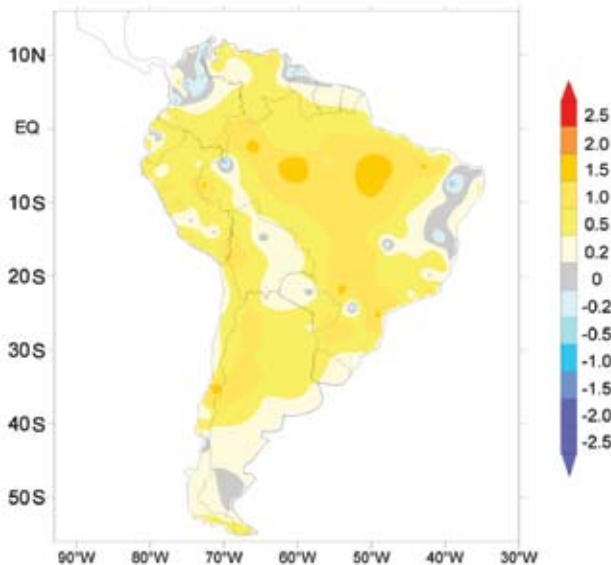
FIG. 6.20. South American 2006 annual temperature anomalies (°C, 1971–2000 base) from CAMS-OPI.
