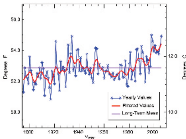
FIG. 6.12. Annual temperature ( ^\circ\text{F} and ^\circ\text{C} ) averaged across the contiguous United States from 1895 to 2006.
