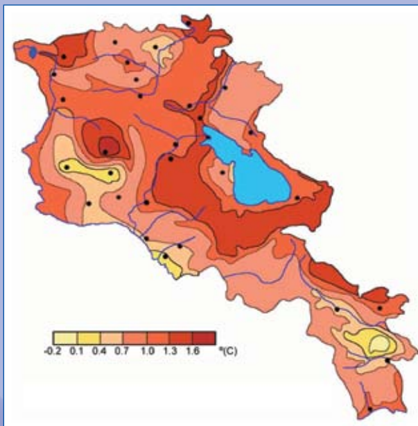
FIG. 6.40. Annual average air temperature (°C) anomalies for Armenia.
