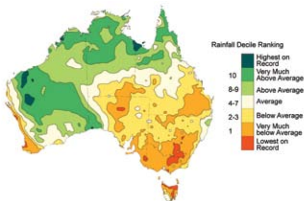
FIG. 6.44. Australian rainfall deciles for 2006 (1900–2006 base).
