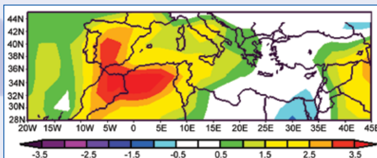
FIG. 6.5. May air temperature anomalies over northwest Africa (°C).
