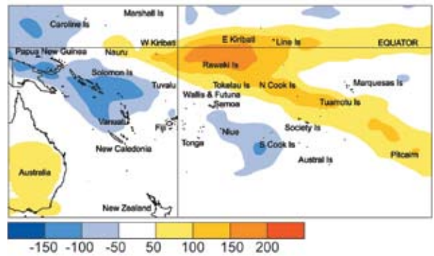
FIG. 6.45. Annual South Pacific OLR anomalies ( \text{W m}^{-2} ). High radiation levels (yellow or orange) are typically associated with clearer skies and lower rainfall, while low values (blue) often indicate cloudy conditions and more rain for the region.
