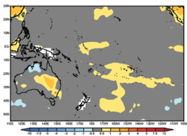
FIG. 6.42. 2006 annual temperature anomalies (°C, 1971–2000 base) for Oceania from CAMS-OPI.
