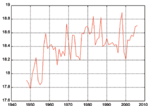
FIG. 6.21. Time series of annually averaged air temperature (°C), spatially averaged from 15°N to 55°S and 30° to 90°W, for the 1948–2006 period. [Source: NCEP–NCAR reanalysis at www.cdc.noaa.gov/cgi-bin/Composites/ .]
