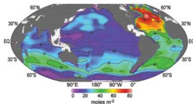
FIG. 3.18. Column inventory of anthropogenic CO 2 (mol m -2 ) that has accumulated in the ocean between 1800 and 1994. High inventories are associated with deep water formation in the North Atlantic and intermediate and mode water formation between 30° and 50°S (Sabine et al. 2004b).
