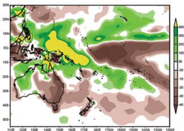
FIG. 6.41. 2006 annual precipitation anomalies (mm, 1979–2000 base) for Oceania from CAMS-OPI.
