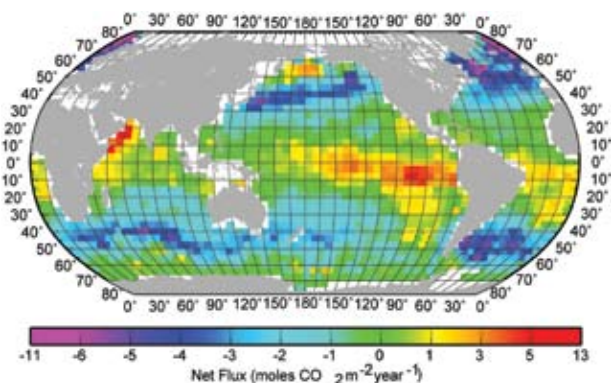
FIG. 3.16. Mean annual net air-sea flux for CO 2 (moles CO 2 m -2 yr -1 ) for the reference year 1995. Red-yellow areas indicate that the ocean is a source for atmospheric CO 2 , and blue-purple areas indicate that the ocean is a CO 2 sink. From Takahashi et al. (2002).
