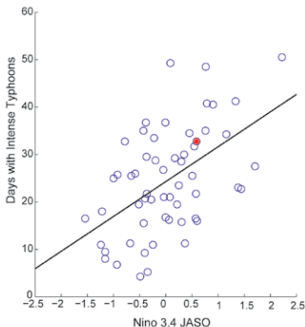
FIG. 4.16. Scatterplot of number of days with intense typhoons and Niño-3.4 index (°C) for JASO in the period 1950–2006; the black line is the linear regression, the number of intense typhoons for 2006 is marked in red ( r = 0.52 ).
