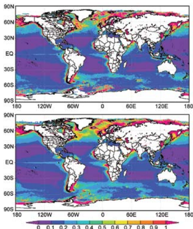
FIG. 3.20. Global time-averaged chlorophyll-a concentration ( \text{mg m}^{-3} ) plots for (top) January–December 2006 and (bottom) September 1997–December 2005. Images generated by NASA's Giovanni ( giovanni.gsfc.nasa.gov ).
