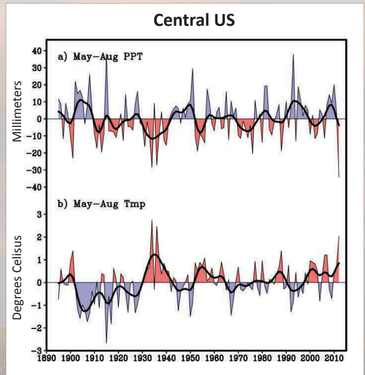
Figure 7. 1895-2012 time series of May-August central Great Plains rainfall departures (mm, top) and surface air temperature departures ( ^{\circ}\text{C} , bottom). Reference period is 1895-2011. Black curve is a 9-point Gaussian filter. The area is comprised of the 6-State region of WY, CO, NE, KS, MO, and IA. Data source is the NOAA U.S. Climate Divisions.
