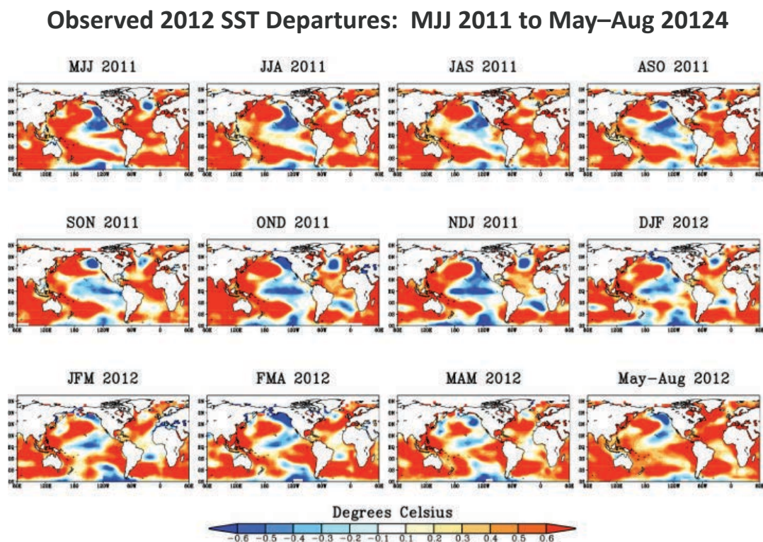
Figure 17. As in Fig. 15, except for the SST anomalies (°C) during the 12-month period antecedent to the occurrence of dry May–August 2012 central Great Plains drought. Reference period is 1901–1990. Data source is the monthly NOAA Merged Land–Ocean surface temperature analysis (MLOS).
