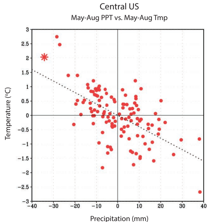
Figure 3. The observed relationship between May-August averaged rainfall departures (mm, x-axis) and surface temperature departures (°C, y-axis) over the U.S. central Great Plains. Reference period is 1895-2012. The 2012 departures are -34mm, and +2.1°C, and shown by the red asterisk. Dashed line is the linear relation between temperature and precipitation variability. Note that for extreme dry conditions, temperatures are appreciably warmer than predicted by this linear fit. May-August departures are averages over the multi-state region (WY, CO, NE, KS, MO, IA). Data source is the NOAA U.S. Climate Divisions.
