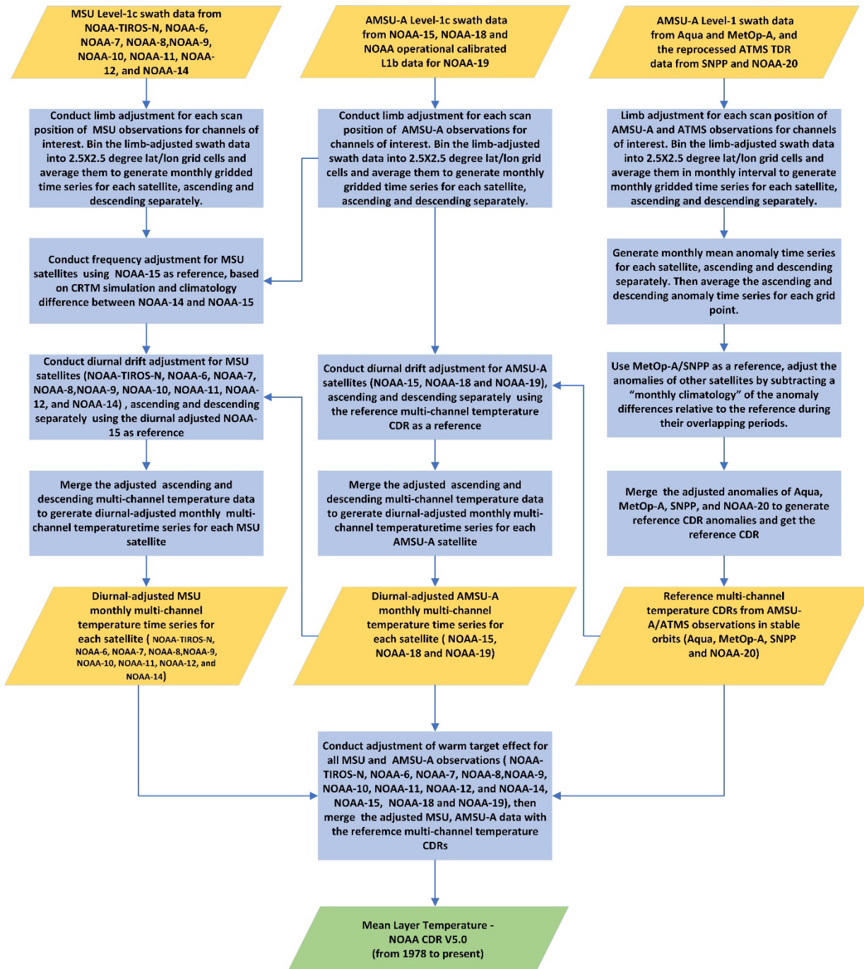
Figure 1. Overall data flow chart of the MLT NOAA CDR V5.0 algorithm.
