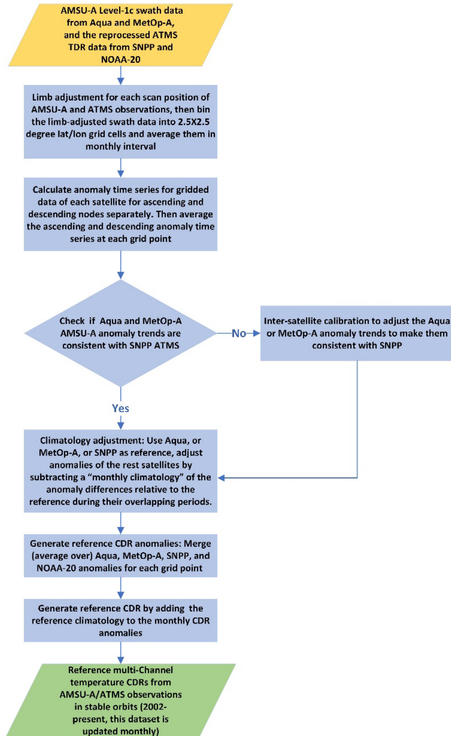
Figure 3. Flowchart for generating reference multi-channel temperature CDRs.
