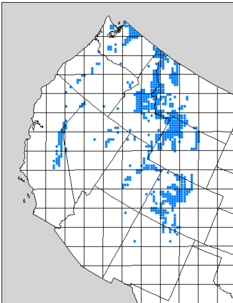
Figure 4: A comparison of IMS daily resolution (blue) to weekly grid cells.
