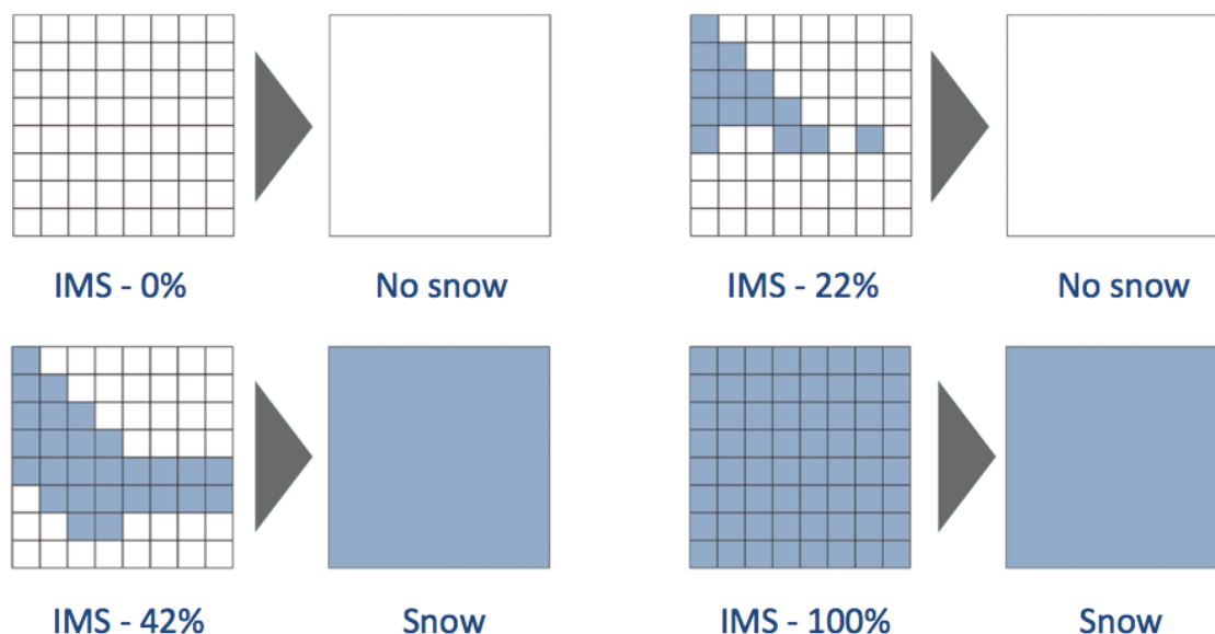
Figure 5: Examples of snow decision from IMS to weekly grid cells.
