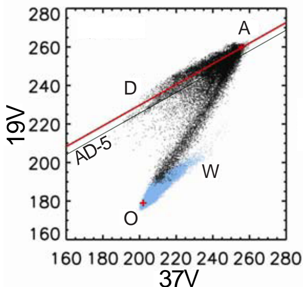
Figure 7: Example of the relationship of the 19V vs. 37V T_B (in Kelvin) used in the Bootstrap algorithm. Brightness temperatures typically cluster around the line segments AD (representing 100% sea ice) and OW (representing 100% open water). For points that fall below the AD-5 line (dotted line), bootstrap uses T_B relationships for 37H vs. 37V. Adapted from Comiso and Nishio (2008).
