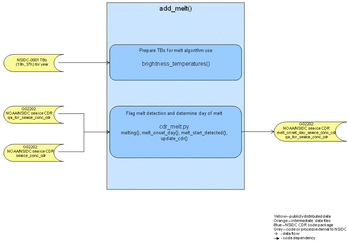
Figure 4: Overview of python code for adding melt start detection.
