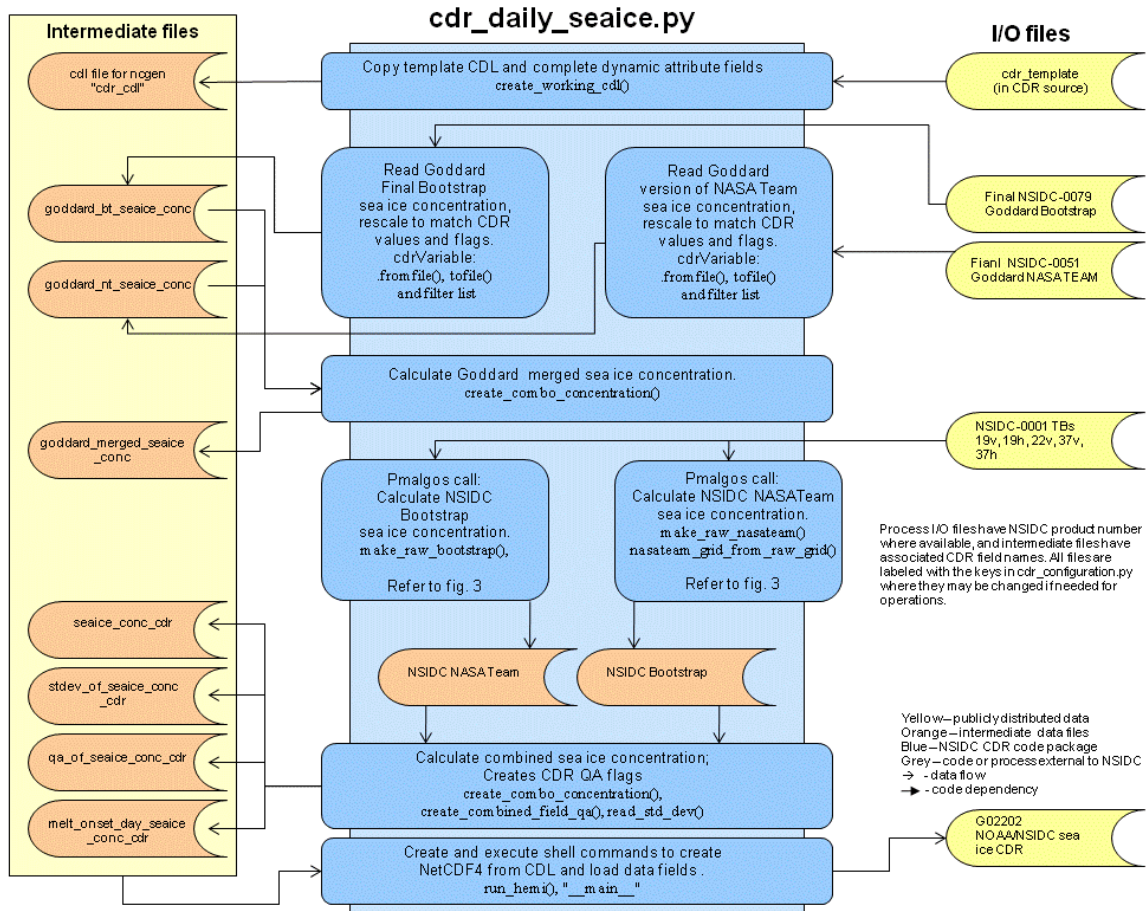
Figure 2: Overview of main python code for the daily sea ice concentration CDR processing.
