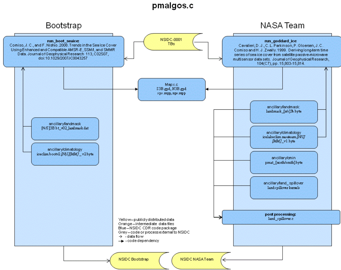
Figure 3: Overview of sea ice CDR algorithm C code.
