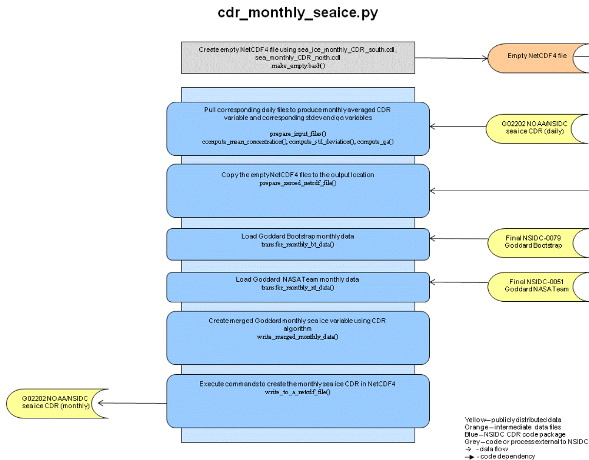
Figure 5. Monthly CDR Processing
