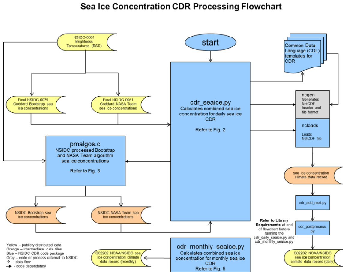
Figure 1: Sea ice concentration CDR processing overview
