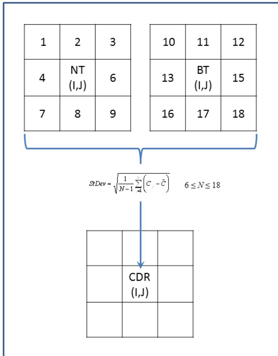
Figure 10: Schematic of grid cell values used in calculation of the CDR standard deviation field. All non-missing ocean/sea ice concentration values ( C ), from both the NASA Team and Bootstrap algorithm, of the 3 \times 3 box surrounding each (I,J) grid cell (up to 18 total values) are used to calculate the standard deviation. A minimum of six grid cells with valid values is used as a threshold for a valid standard deviation.
