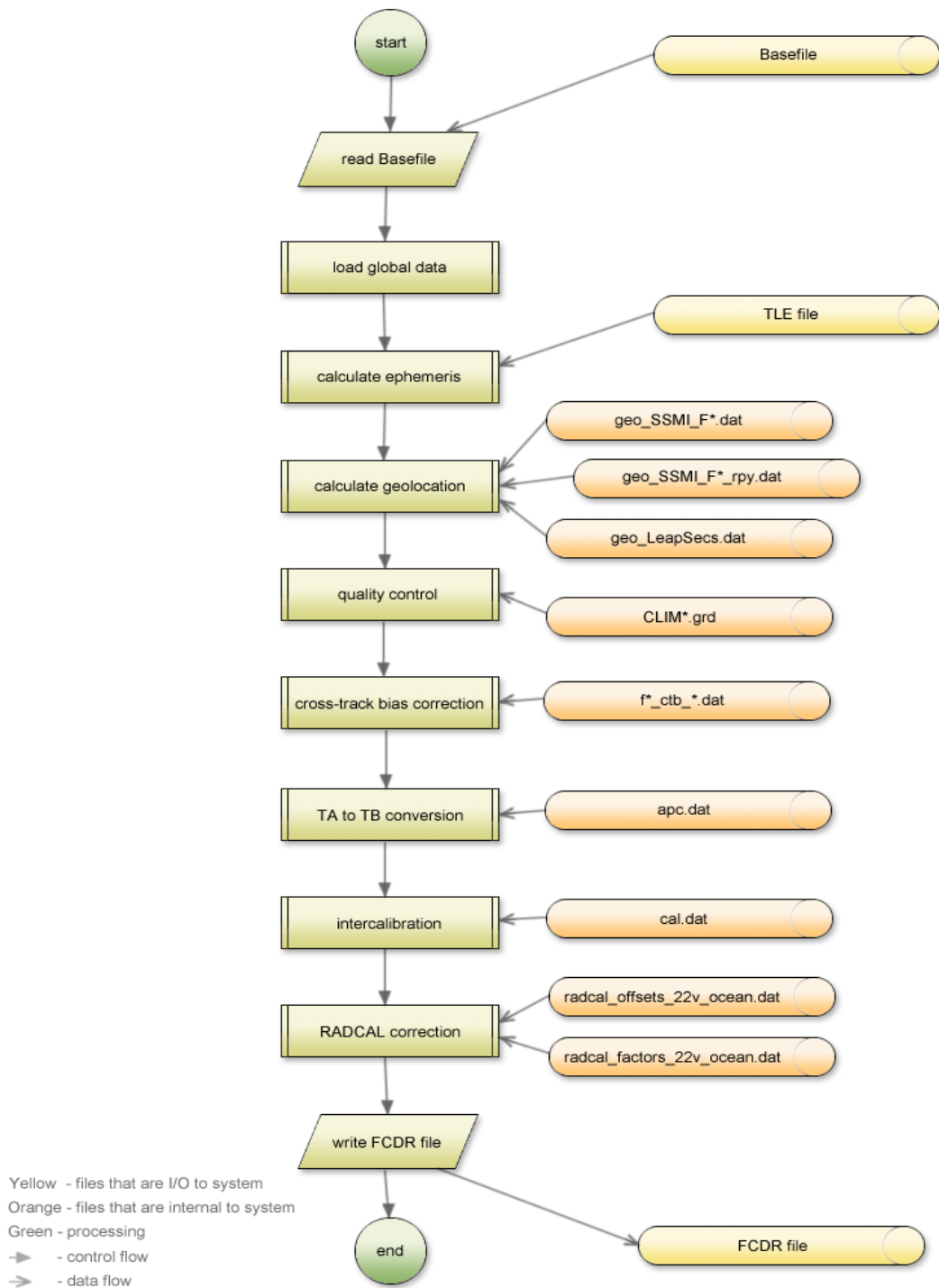
Figure 2: FCDR for SSM/I Outline Processing Flowchart.
