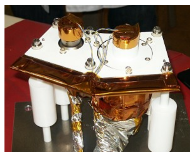
Figure 10 : OSTM/Jason-2 T2L2 Optics Unit
