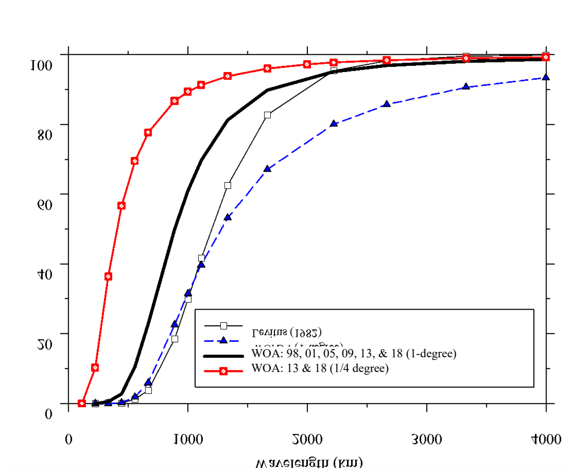
Figure 2. Response function of the WOA18, WOA13, WOA09, WOA05, WOA01, WOA98, WOA94, and Levitus (1982) objective analysis schemes.
