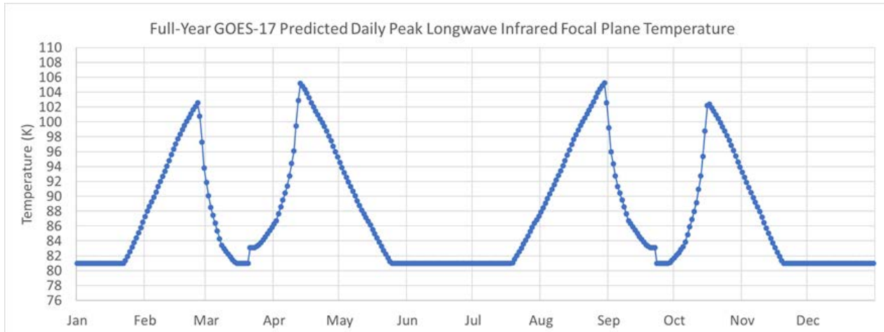
Figure 1. GOES-17 predicted daily maximum longwave focal plane module (FPM) temperature. Courtesy of Harris Corporation. These are approximate maximum daily FPM temperatures. The plot demonstrates the annual seasonal pattern expected due to the warming of the instrument. On a given day, the FPM temperature is stable around 81K most of the day and is only elevated for part of the night. That period varies with the seasons, with the longest duration (~9 hours) on the hottest peak days of the year and the shortest duration (~3 hours) during the coolest peak days. The cooling due to spacecraft eclipse by Earth during the vernal and autumnal equinox are apparent. The estimated times when yaw flips will occur during the equinoxes are seen as sharp discontinuities in March and September. In general, the hotter the FPM temperature, the larger the impact on ABI bands 8-16 quality and ultimately, availability.
