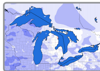
Water level statistics based on 1918-2016.
